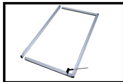
Connect bottom 2' bar and other vertical corner bar. Repeat to create opposite side end frame
